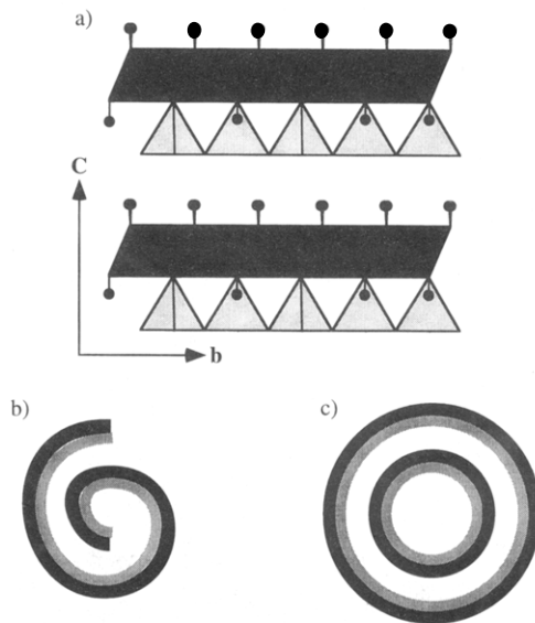
Figure 2. The idealized structure of chrysotile: (a) The lizardite structure viewed down the a -axis (the triangles represent the silicon–oxygen tetrahedra and the darker layers, the \text{Mg}(\text{OH})_2 octahedral sheet); (b) the chrysotile structure based on rolled lizardite layers (darker band is the octahedral sheet); and (c) the chrysotile structure based on concentric lizardite layers. Structural diagram courtesy of G. D. Guthrie, Jr. (Los Alamos National Laboratory, Los Alamos, NM).
